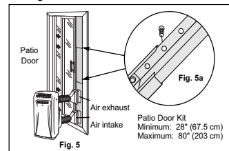
Plug the unit into a 115 V / 60 Hz grounded electrical outlet.
