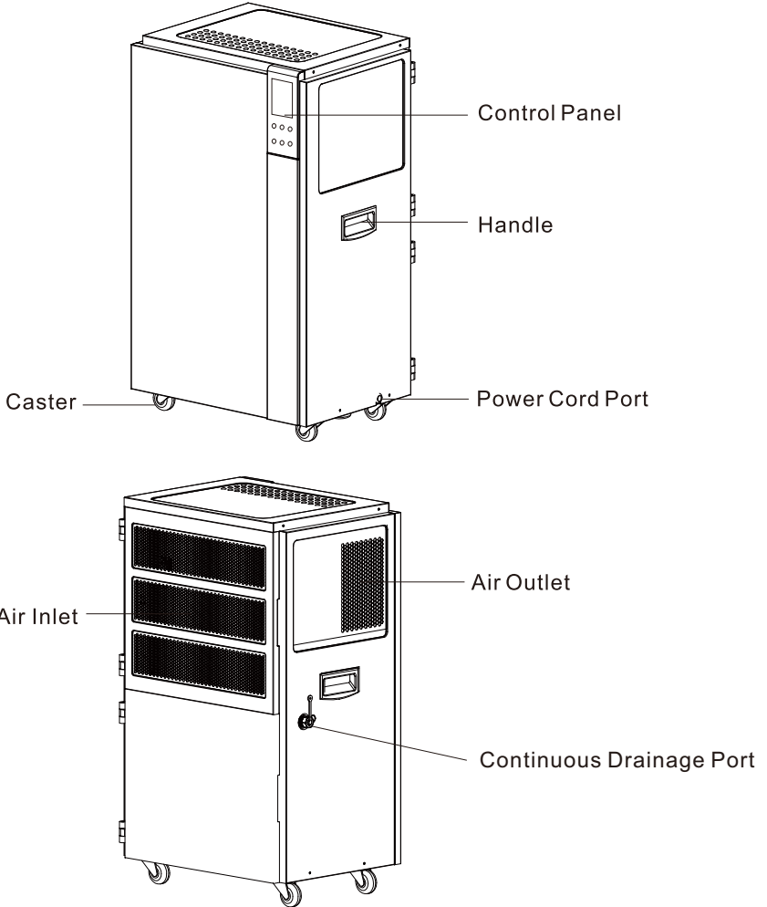
Schematic Diagram
